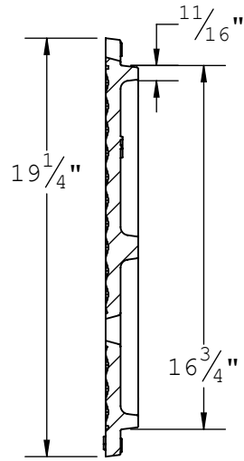
SECTION C-C
