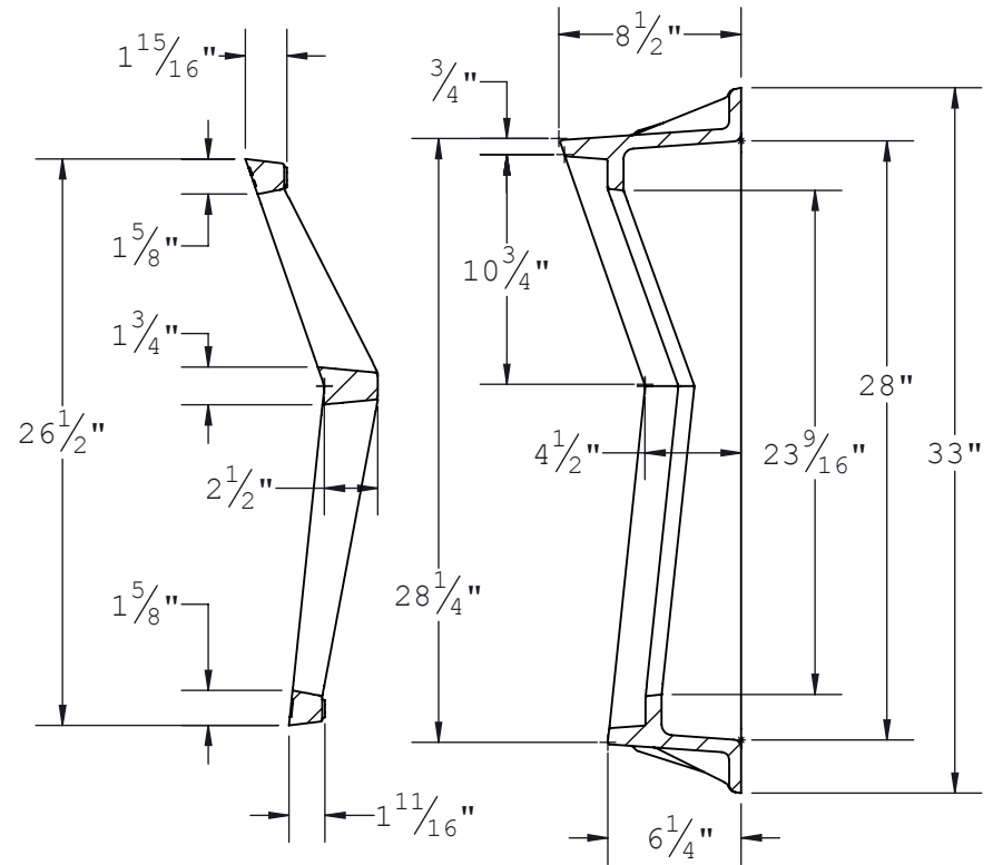
SECTION B-B
